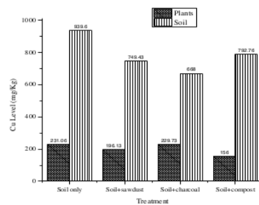
Figure 2. Copper level comparison in the soil and plant. The average of Cu distribution level in the soil-plant system within the lisimeter treated with sawdust, charcoal and compost is lower than controlled lisimeter (soil only).
